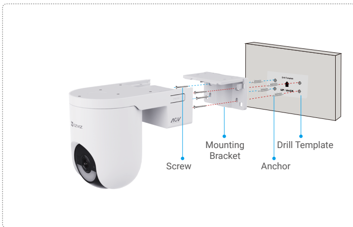
Fig. 2 Wall Mount
